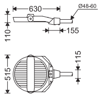
M313U...+GPDS5-Bracket M313U...+GPDS6-Bracket
