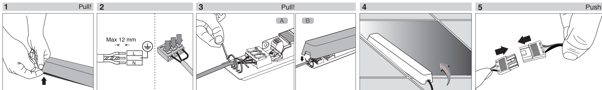
Mounting the panel in exposed T-grid false ceiling
