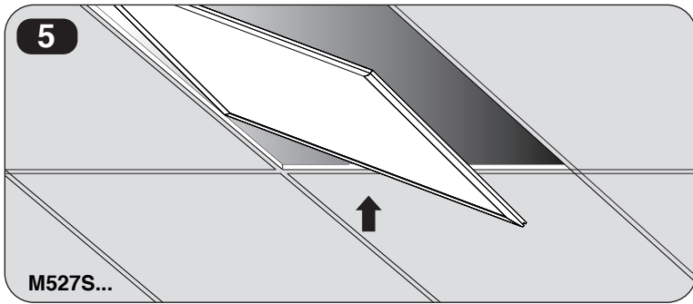
Mounting the panel in exposed T-grid false ceiling
