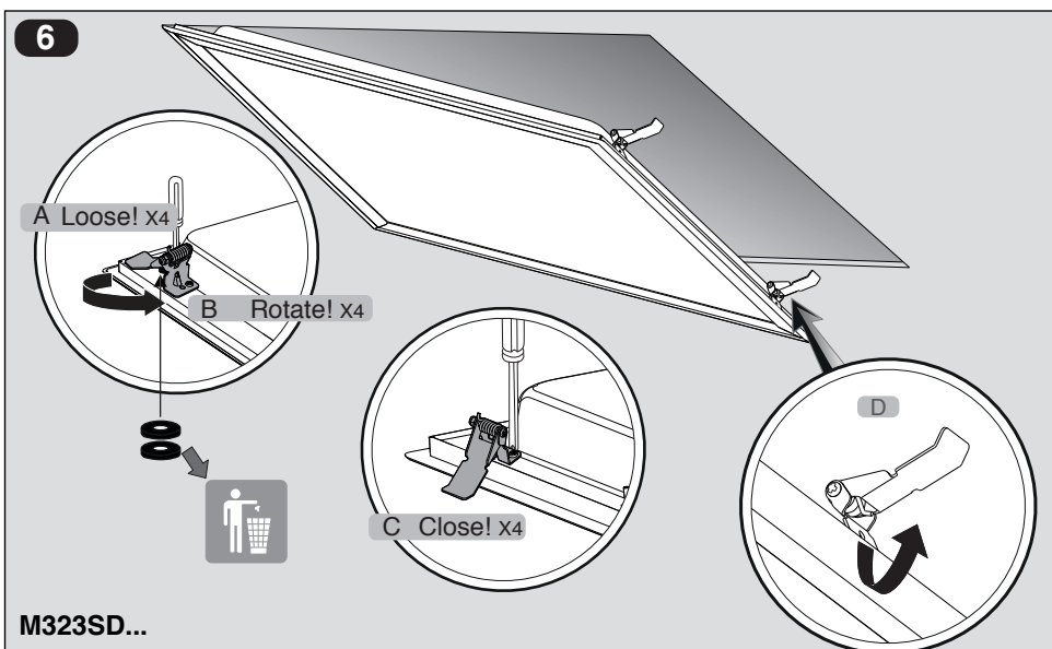
Mounting the panel in exposed T-grid false ceiling
