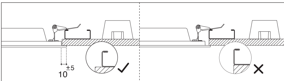
Mounting the LED panel in gypsum false ceiling
