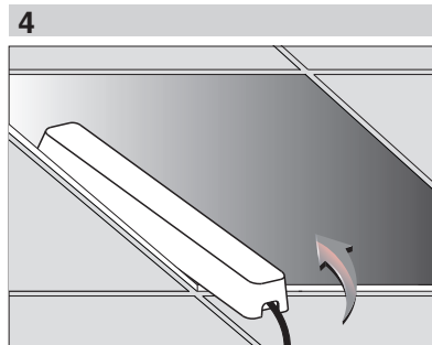
Mounting the panel in exposed T-grid false ceiling
