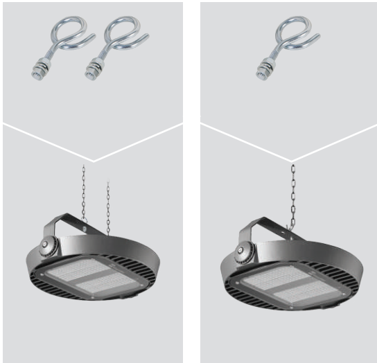
Suspension of the luminaire with one or two provided suspension brackets
